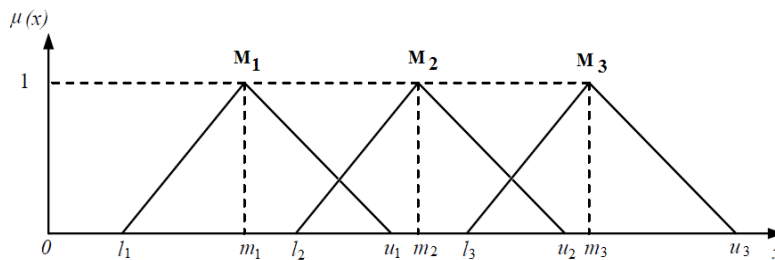
Figure 2. Membership functions for linguistic variables
