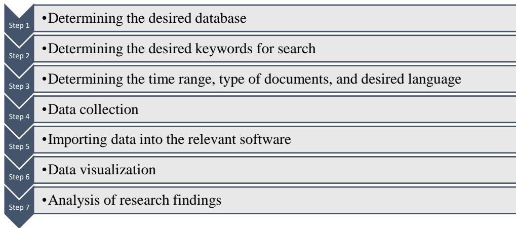
Figure 1. Research steps
