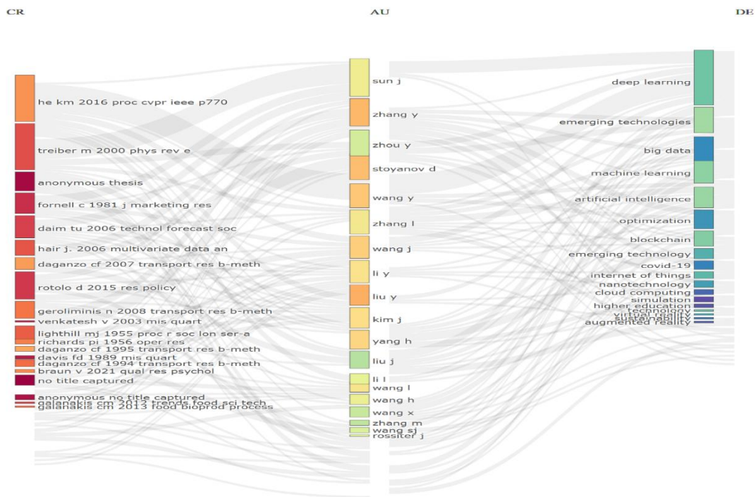
Figure 8. Three-field plot
