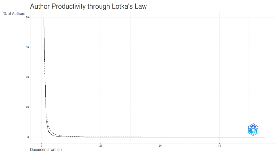
Figure 10. Lotka's Law
