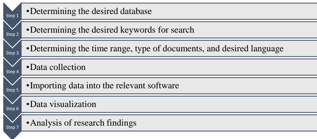
Figure 1. Research steps
