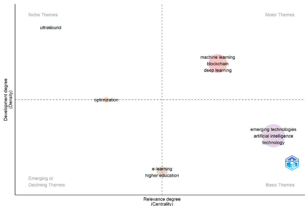
Figure 12. Thematic map
