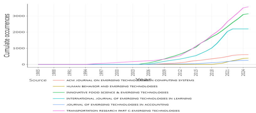
Figure 3. Source dynamics
