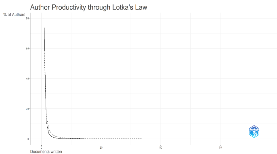
Figure 10. Lotka's Law
